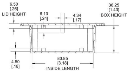
SECTION A-A SIDE VIEW
